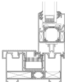
Cill Detail
