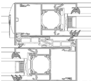
Interlock Detail
